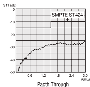
Return Loss for MCVJ-W
