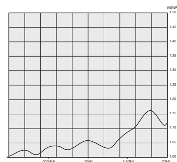
VSWR for CCx7-F
