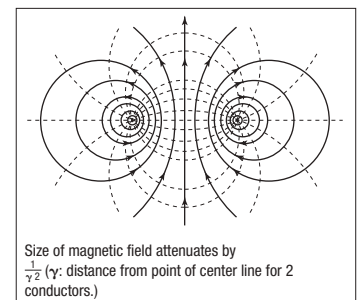
Two-conductor cable
