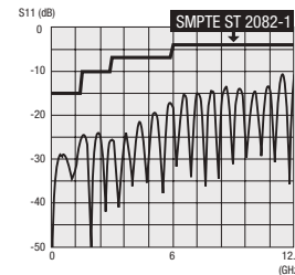
Return loss for HBCP-D25HD
