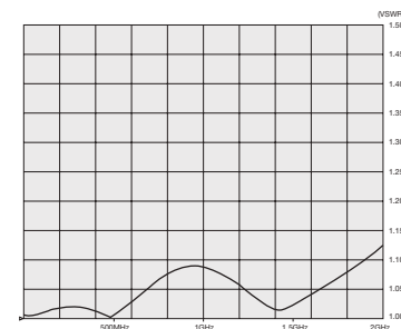
VSWR for CCx4-K
