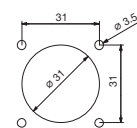
Panel Hole Dimensions
