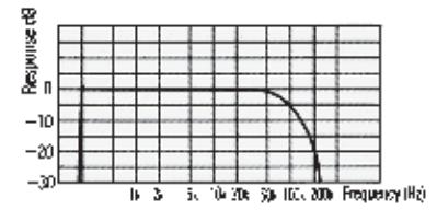
Fig. 2 Frequency Characteristics for L-2B2AT (100m)
