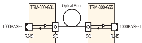
Block Diagram of TRM-300-G31 and TRM-300-G55
