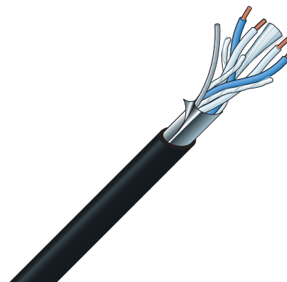
Star quad cable with aluminum foil shield
