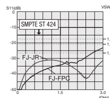
Fig.1 Return loss for FJ-FPC and FJ-JR
