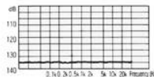
Fig. 1 Crosstalk Characteristics for L-4E4-4AT (100m)
